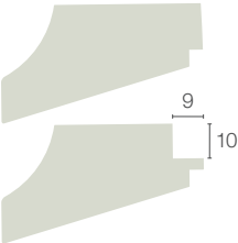
Frame Moulding BG07-1 2,400×63×28 Frame Moulding BG07A-1(Groove Not Included)
