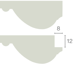
Frame Moulding BG08-1 2,400×60×17
